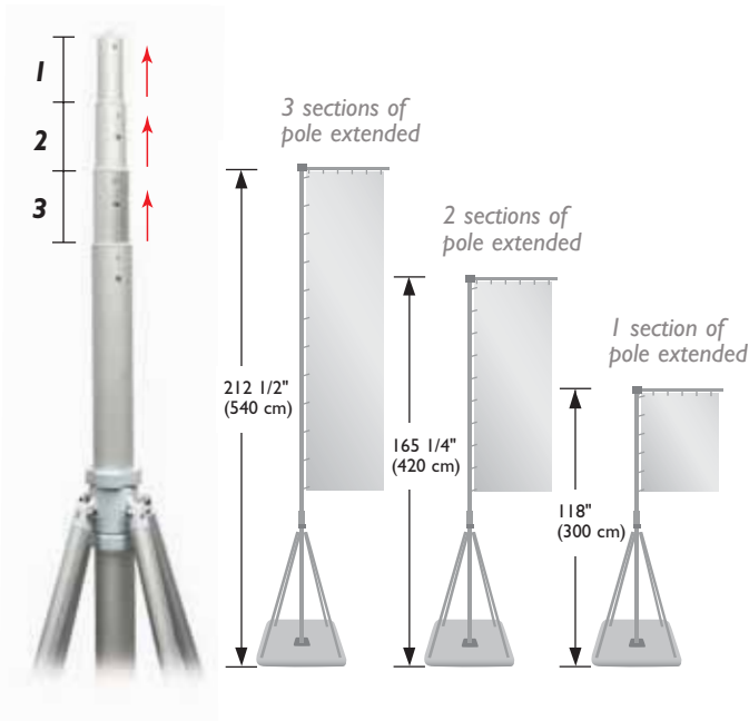
To extend one section of the pole, simply pull up the pole until the pole stop pops up to lock into place.
