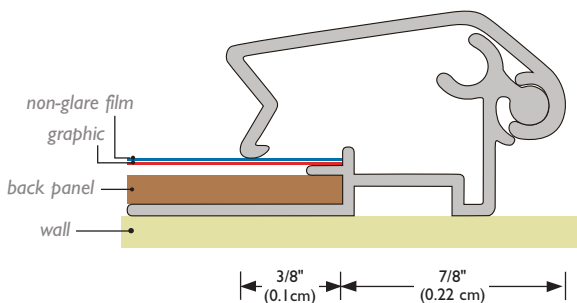
Standard frame with back panel:
